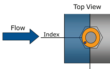
Figure 17. Proper flow switch indexing
