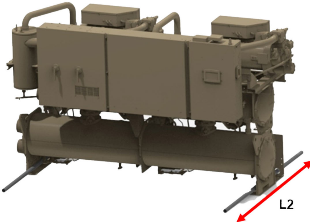
Figure 6. RTWD – anti tipping
