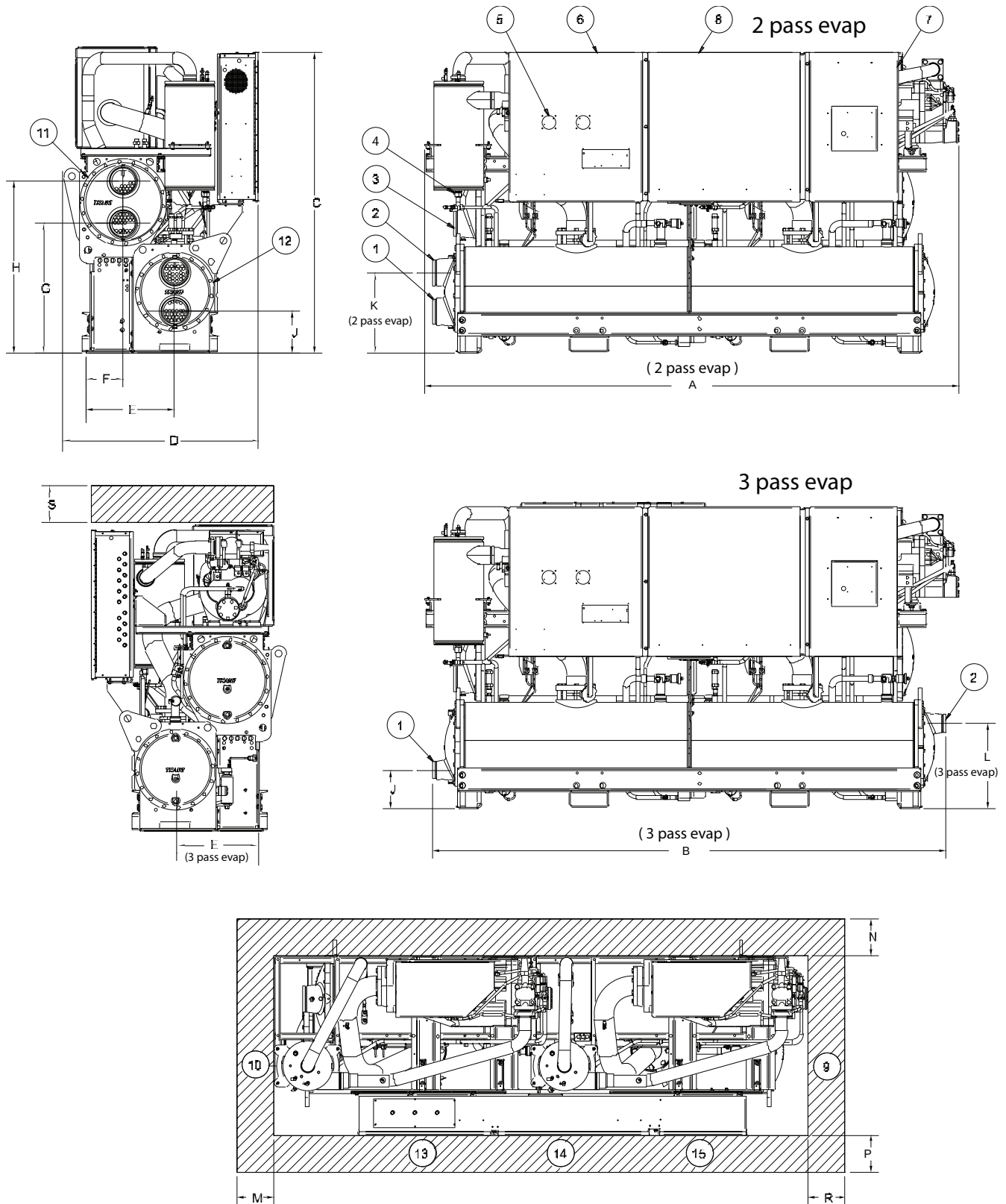
Figure 2. RTWD, 150 to 250 tons, 60 Hz
