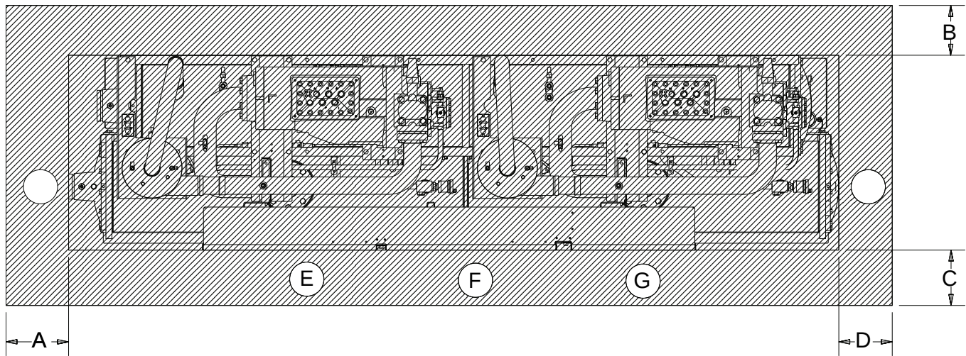
Figure 4. RTWD service clearances
