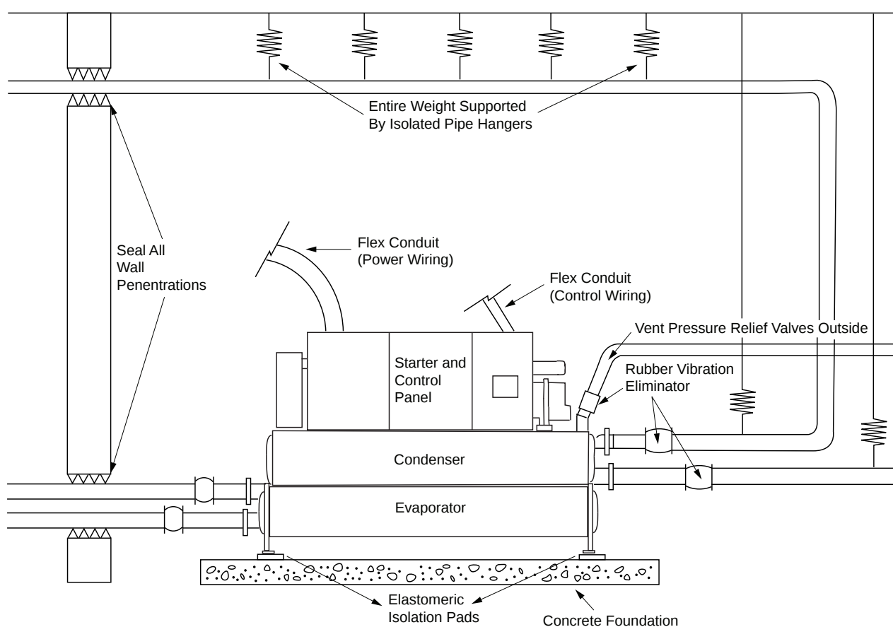
Figure 15. RTWD installation
