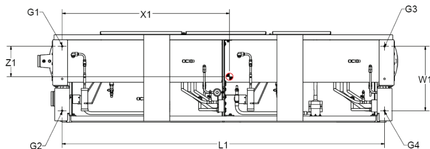
Figure 12. Mounting point locations and weights – RTWD Std efficiency (all), RTWD High efficiency: 80 - 120T (60 Hz)
