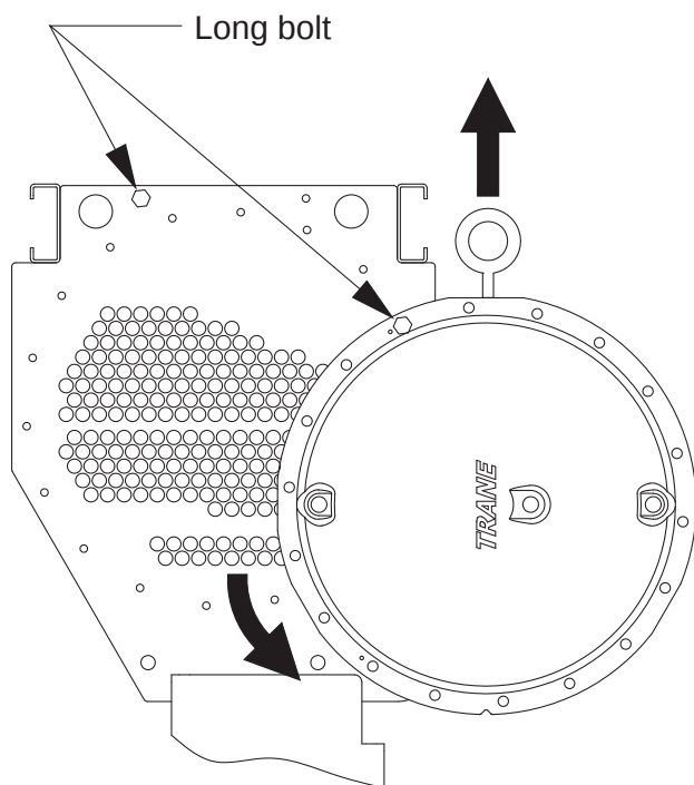
Figure 34. Waterbox removal - swing out, install lifting chain
