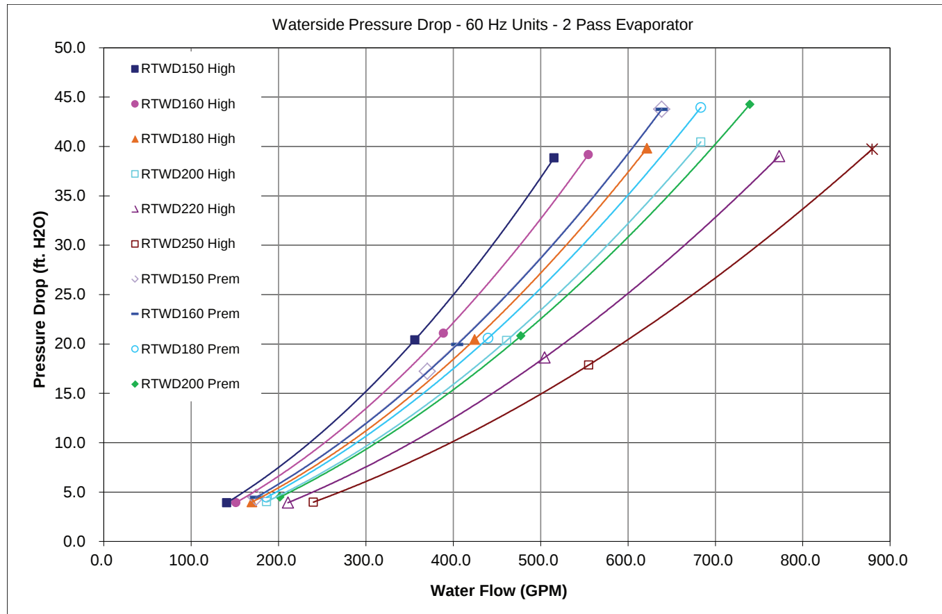
Figure 19. Evaporator pressure drop curves - 2 pass, 60 Hz - RTWD
