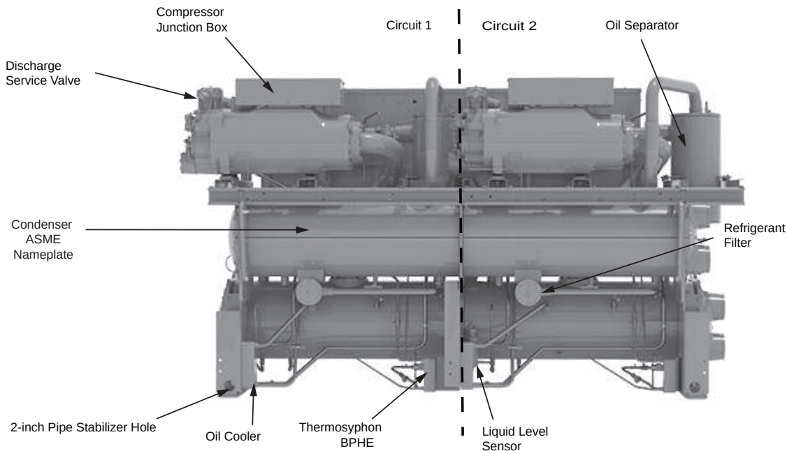
Figure 28. RTWD components – back view
