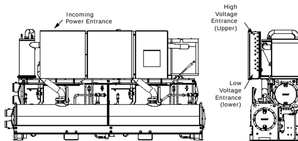
Figure 25. Power entrance
