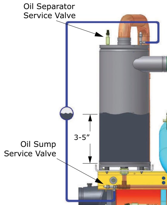
Figure 35. Determining oil level in the sump
