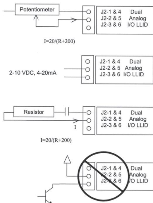
Figure 26. Wiring examples for EDLS and ECWS/EHWS
