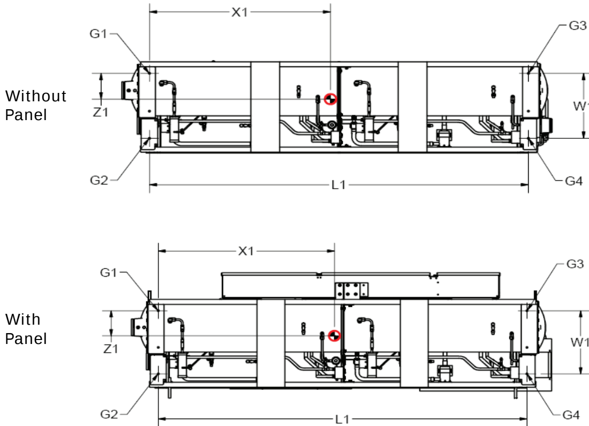
Figure 13. Mounting point locations and weights – RTWD Premium efficiency (all), RTWD High efficiency: 150 – 250T (60 Hz)
