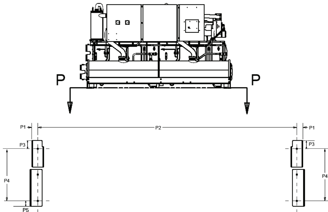
Figure 3. RTWD unit footprint
