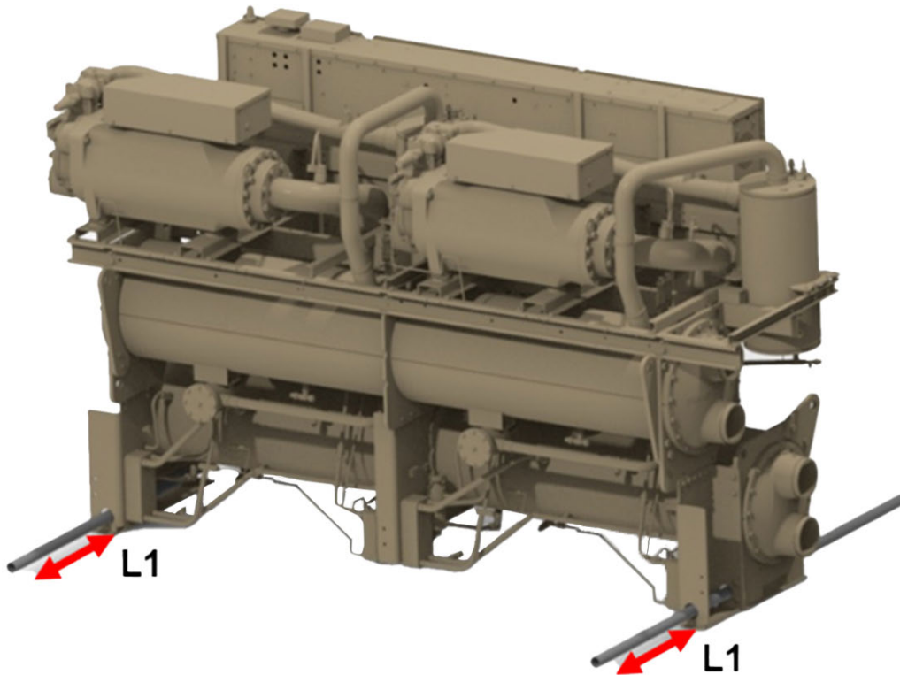
Figure 6. RTWD – anti tipping
