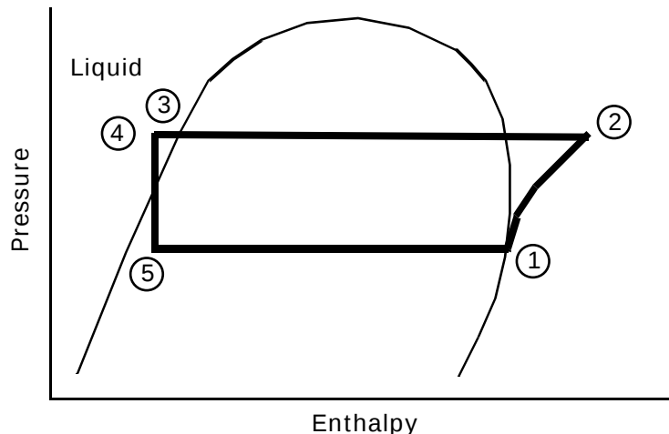
Figure 29. Pressure enthalpy curve
