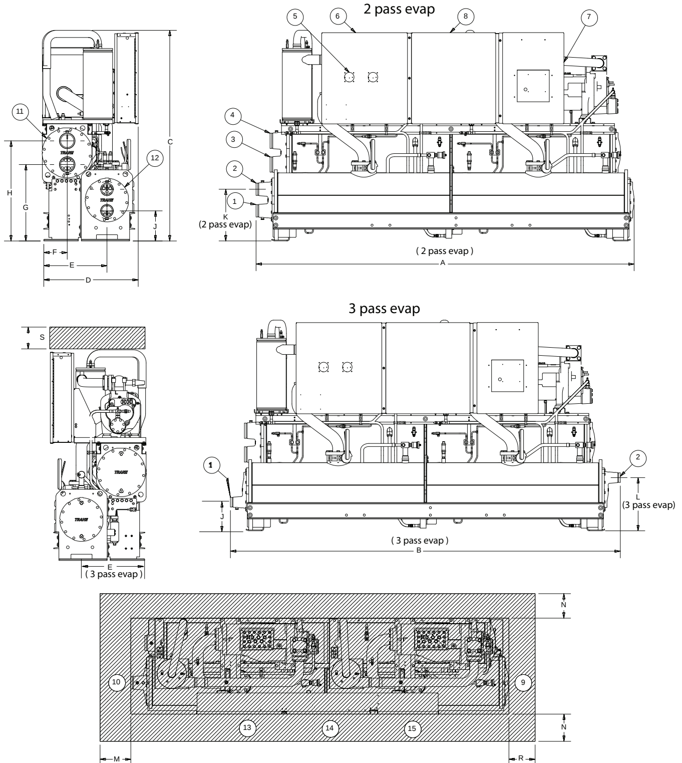
Figure 1. RTWD 80 to 140 tons, 60 Hz
