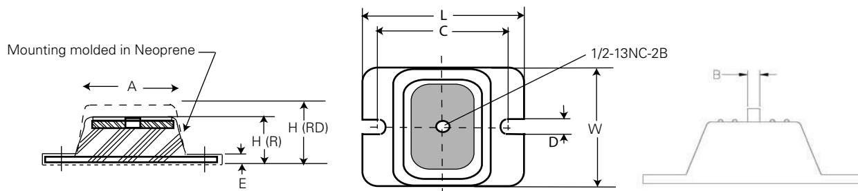
Figure 11. RTWD neoprene isolator
