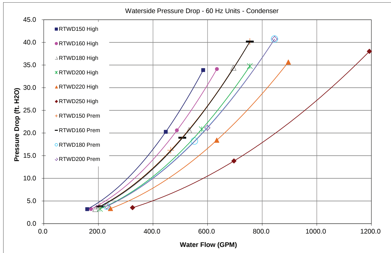
Figure 23. Condenser pressure drop curves - RTWD 60 Hz
