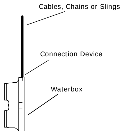
Figure 31. Waterbox lifting
