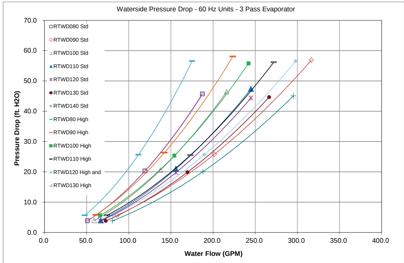
Figure 21. Evaporator pressure drop curves - 3 pass, 60 Hz - RTWD
